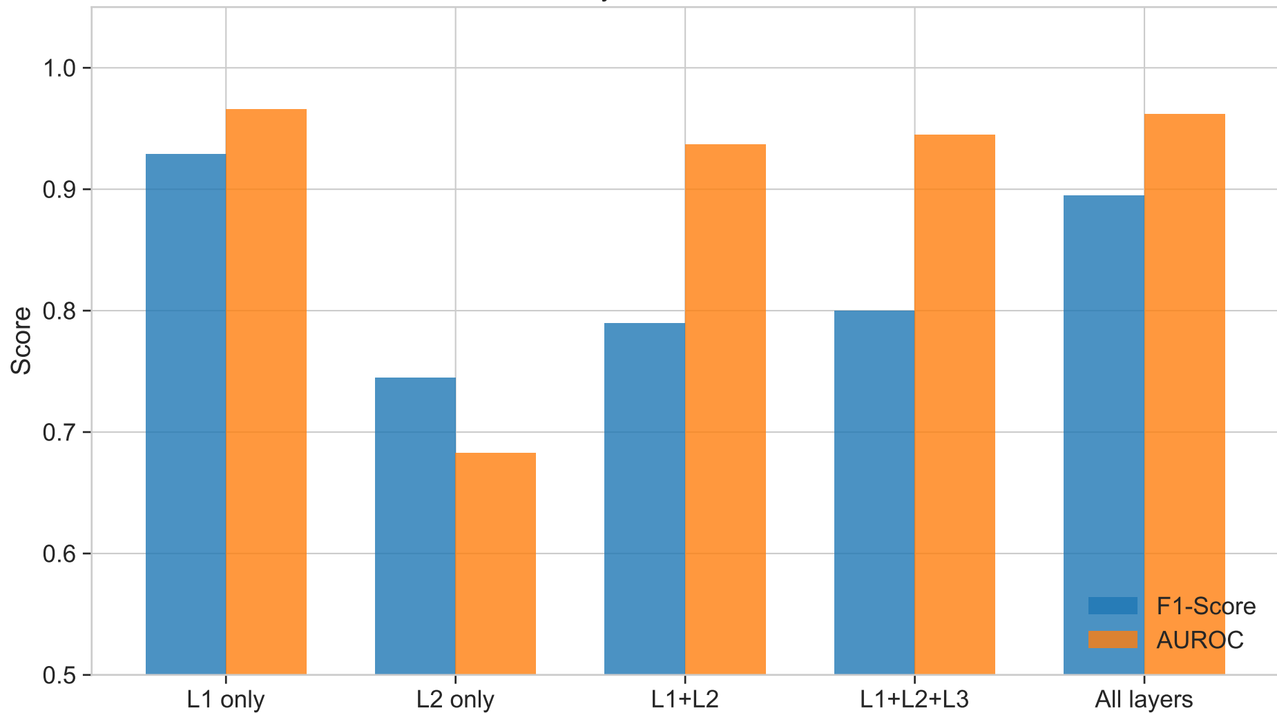
Feature Layer Ablation Performance
